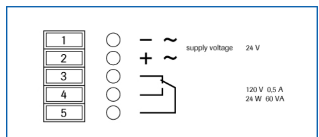
Fig. 3: Receiver
